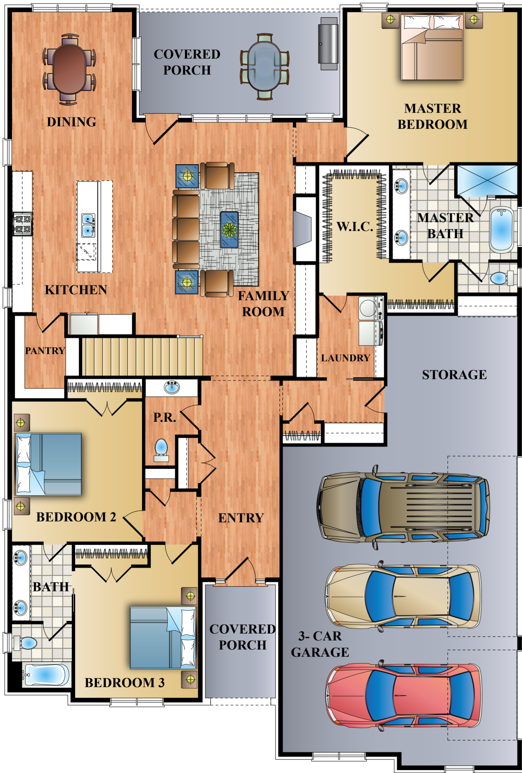
120 STONE RIVER ROAD 1ST LEVEL FLOORPLAN
