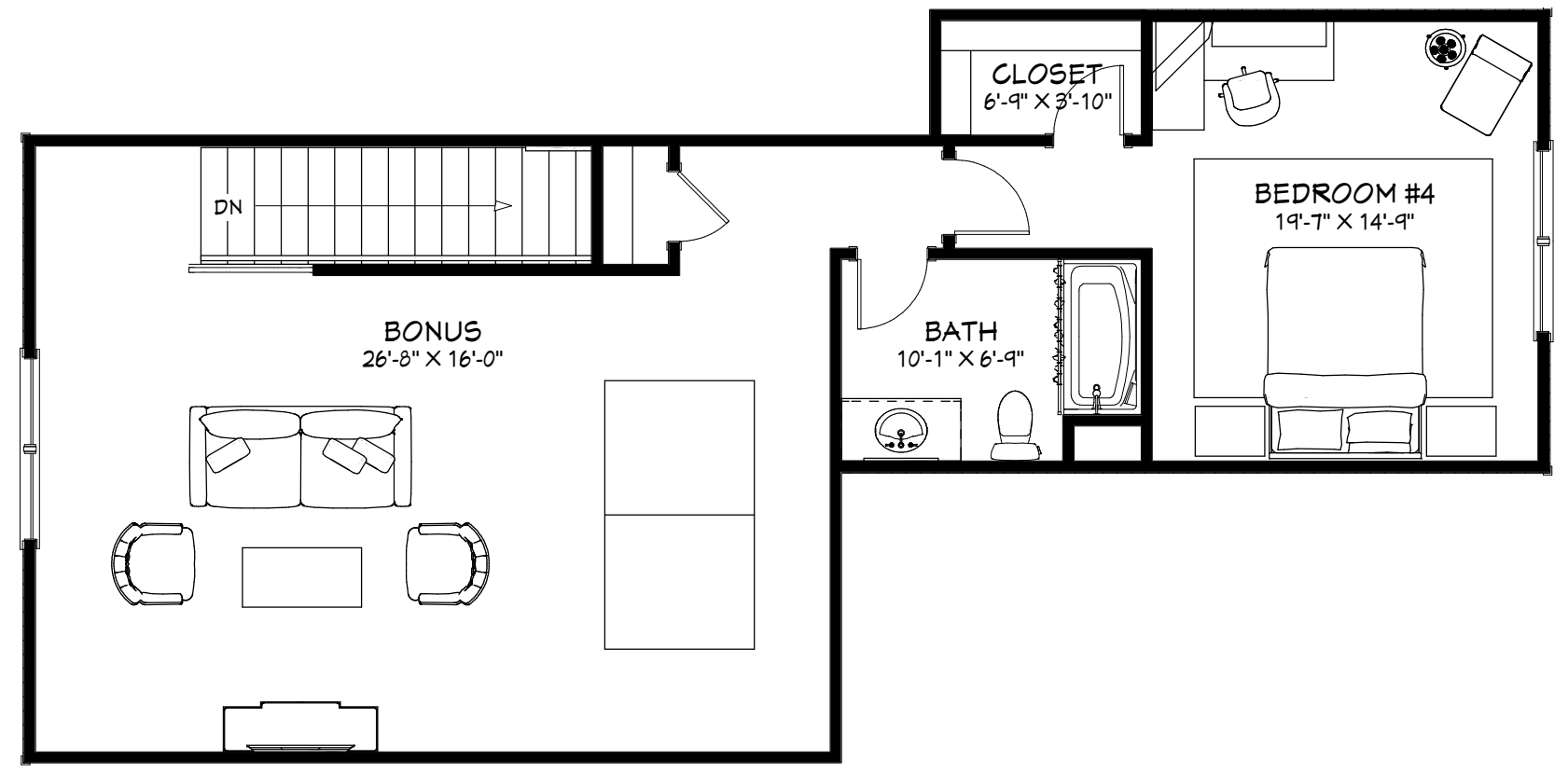
SECOND FLOOR
